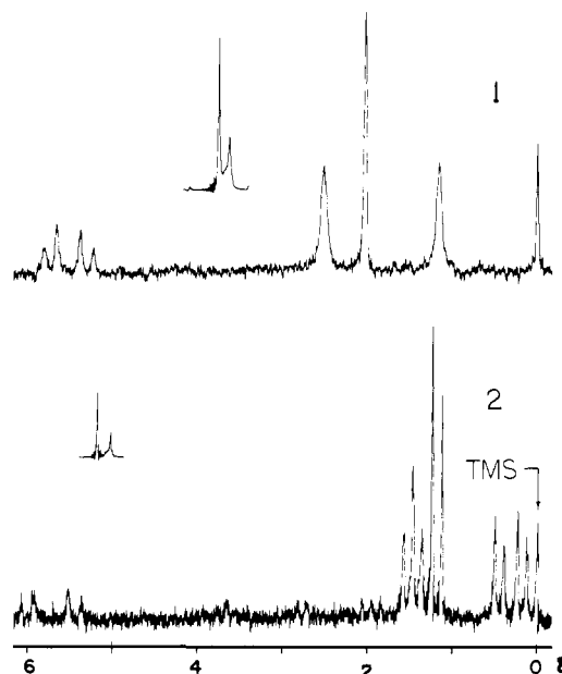
Figure 1. NMR spectra at 500-Hz sweep width of hydrocarbons cis -1-phenyl-2-mesitylacenaphthene (1) and cis -1-phenyl-2-tipylacenaphthene (2) in TCB solution at 200 °C (Me 4 Si internal reference, ethylene glycol temperature calibration).
